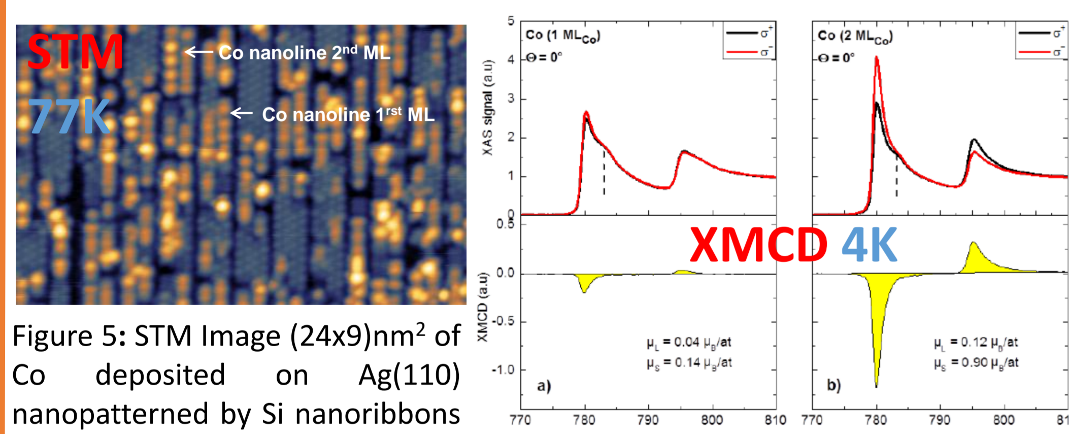
Figure 6: XAS spectra taken at normal incidence ( \Theta = 0^\circ ) for both helicities ( \sigma^+ and \sigma^- ) at 4 K with a magnetic field of 6 T and corresponding XMCD signals for (a) 1 ML Co and (b) 2 ML Co on Si/Ag(110). Orbital and spin magnetic moments in both structures were determined by applying the sum rules.
